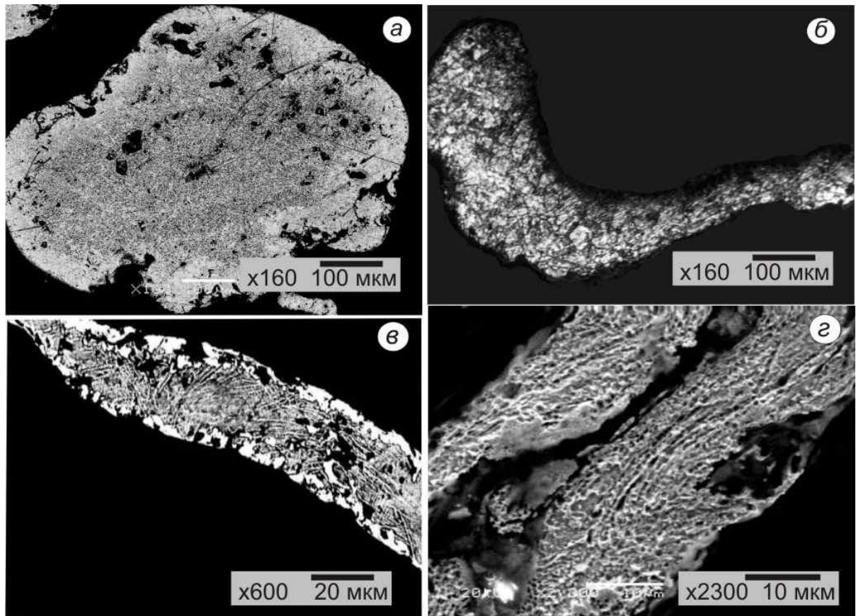
Fig. 3. Inner structure of placer gold: a, b – recrystallized structures; c, d – structures of plastic deformations.
