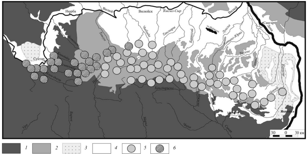
Fig. 1. Diagram of geological structure of the Lena-Viluy syncline. 1 – Jurassic deposits, J; 2 – Cretaceous deposits, C; 3 – Neogene deposits, N; 4 – Quaternary deposits, Q; 5 – Locations of placer gold sampling; 6 – Locations of placer gold sampling with identified Au-Pt mineralization.
