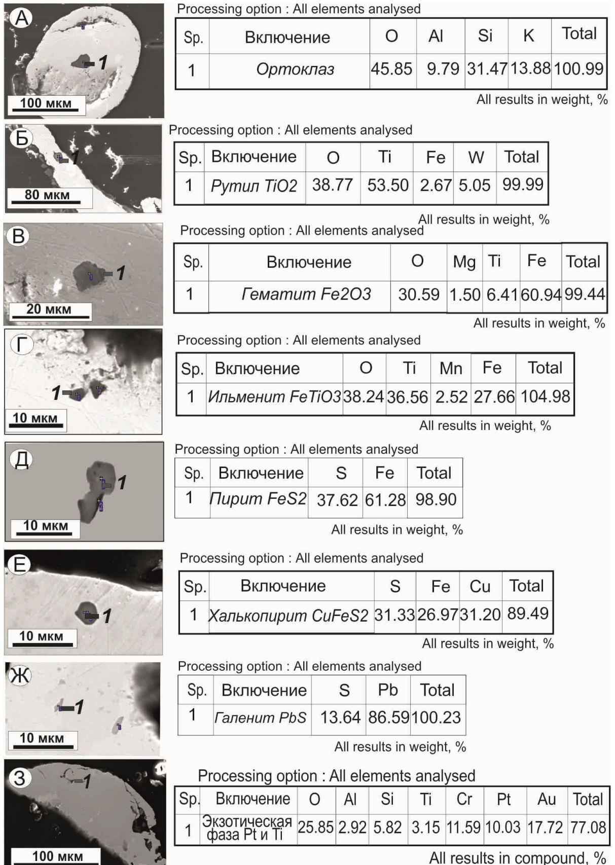
Fig. 2. Micromineral inclusions in placer gold.
